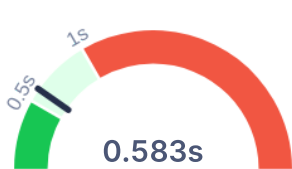
Server Response
